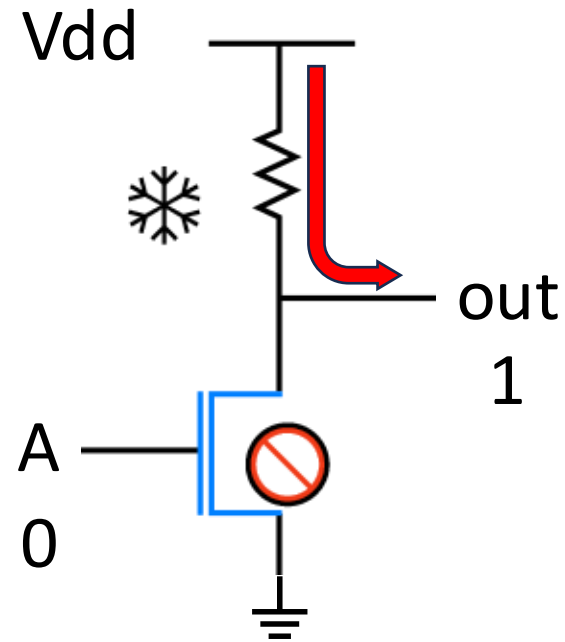
NMOS - 1978
