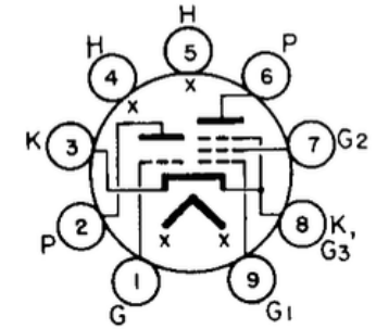
BOTTOM VIEW BASING DIAGRAM JEDEC 9GF
